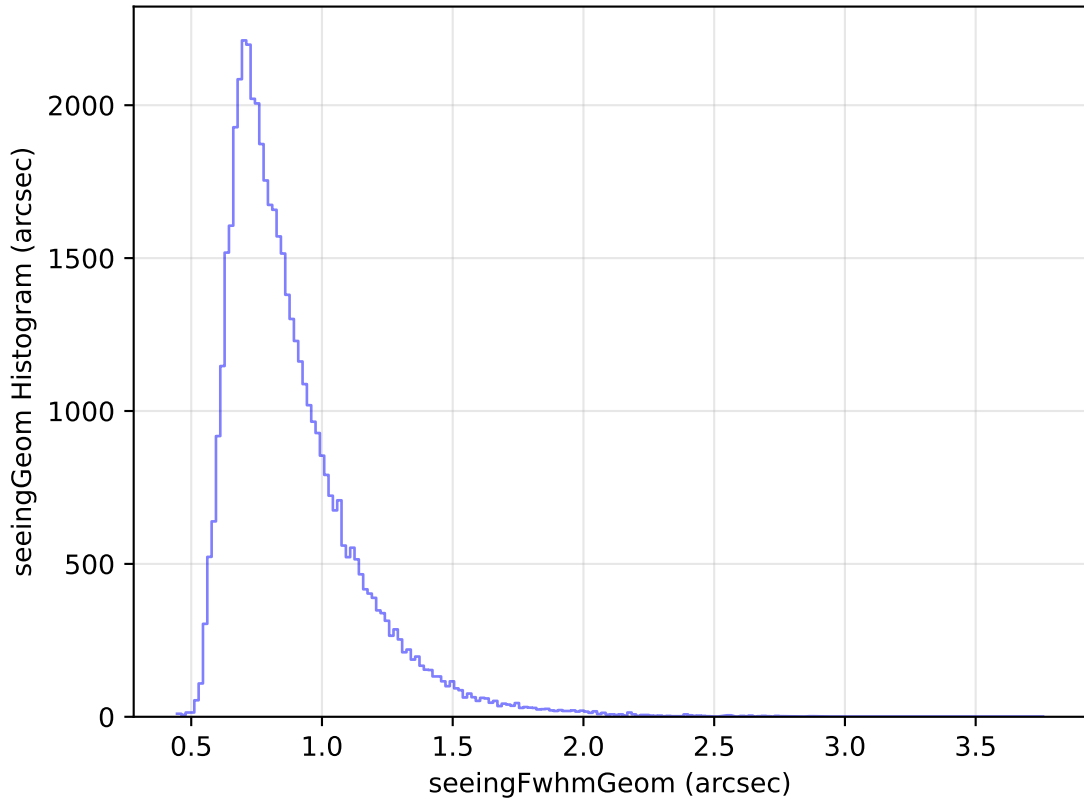
internal_u_expt27_nscale1.2v3.4_10yrs Yr 1 r band: seeingGeom Histogram
