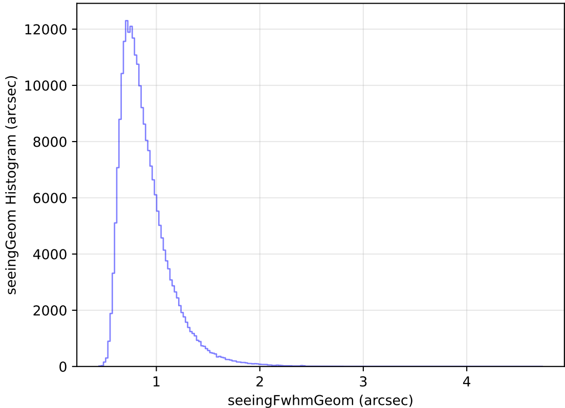
internal_u_expt27_nscale1.2v3.4_10yrs Yr 1 all bands: seeingGeom Histogram
