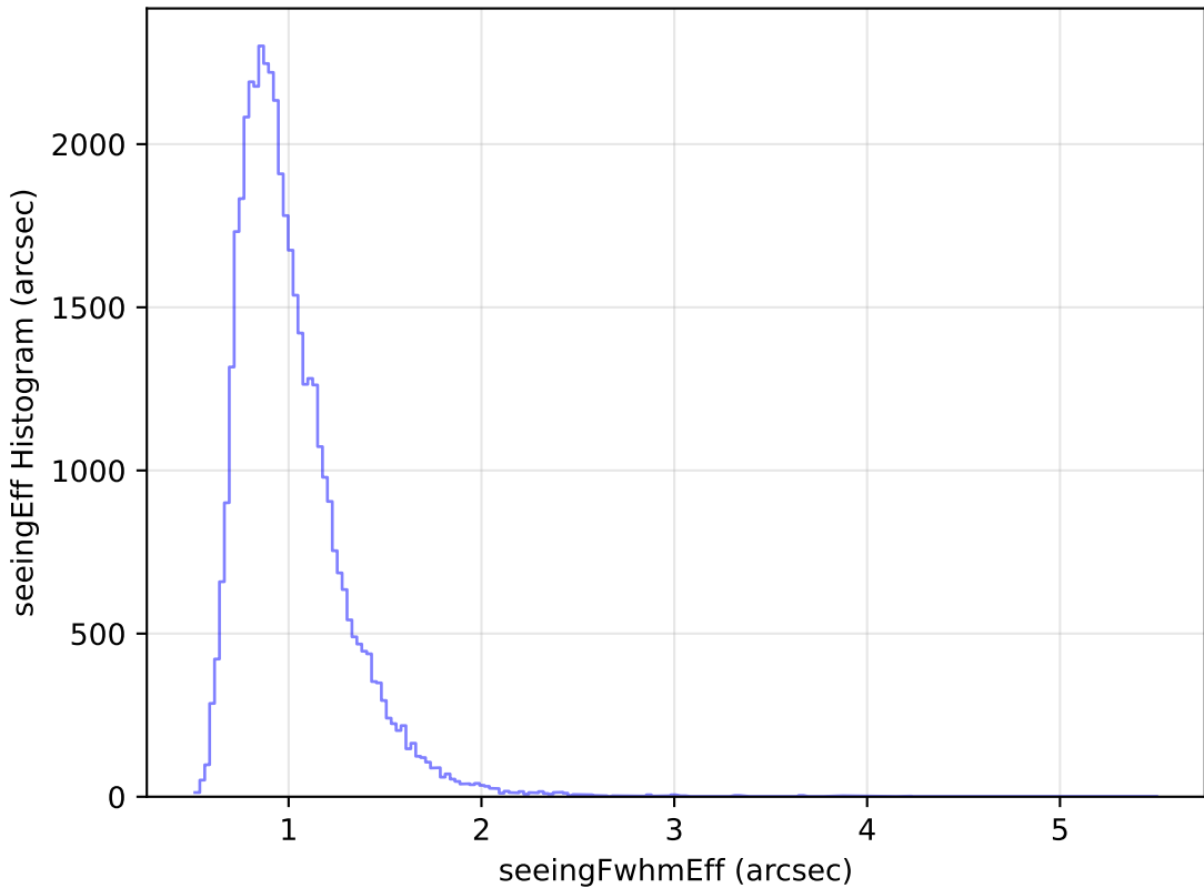
internal_u_expt27_nscale1.2v3.4_10yrs Yr 1 z band: seeingEff Histogram
