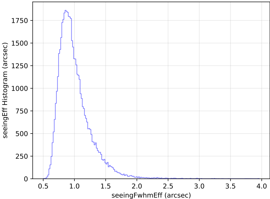
internal_u_expt27_nscale1.2v3.4_10yrs Yr 1 y band: seeingEff Histogram
