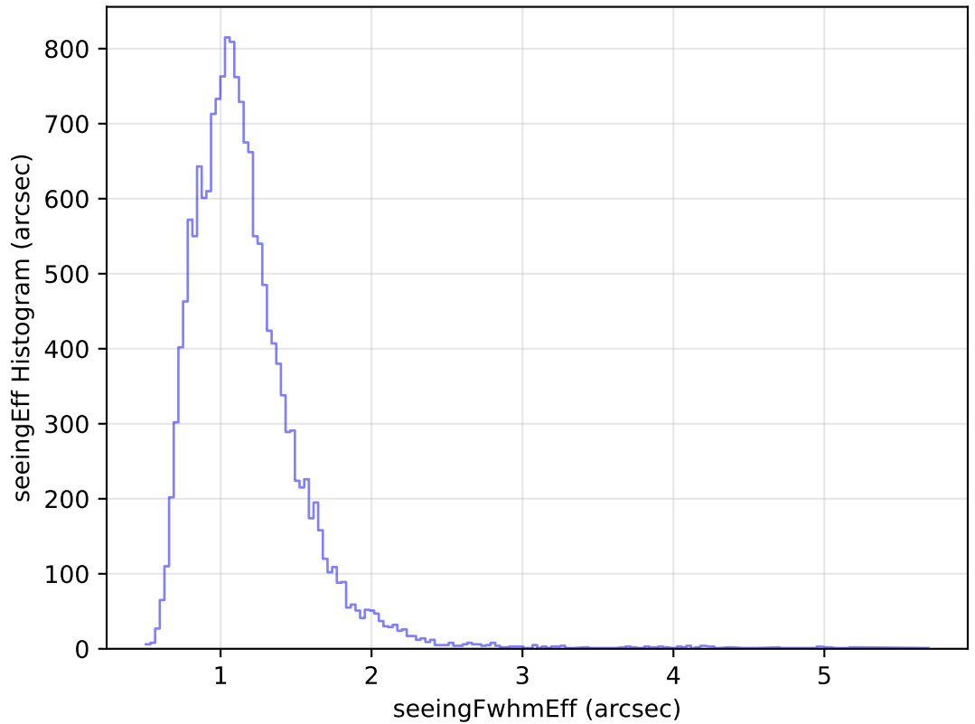
internal_u_expt27_nscale1.2v3.4_10yrs Yr 1 u band: seeingEff Histogram
