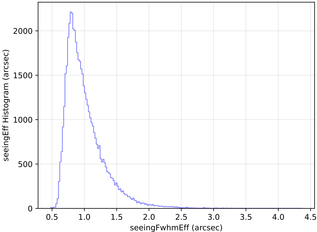
internal_u_expt27_nscale1.2v3.4_10yrs Yr 1 r band: seeingEff Histogram
