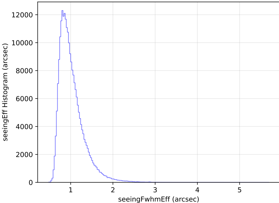
internal_u_expt27_nscale1.2v3.4_10yrs Yr 1 all bands: seeingEff Histogram
