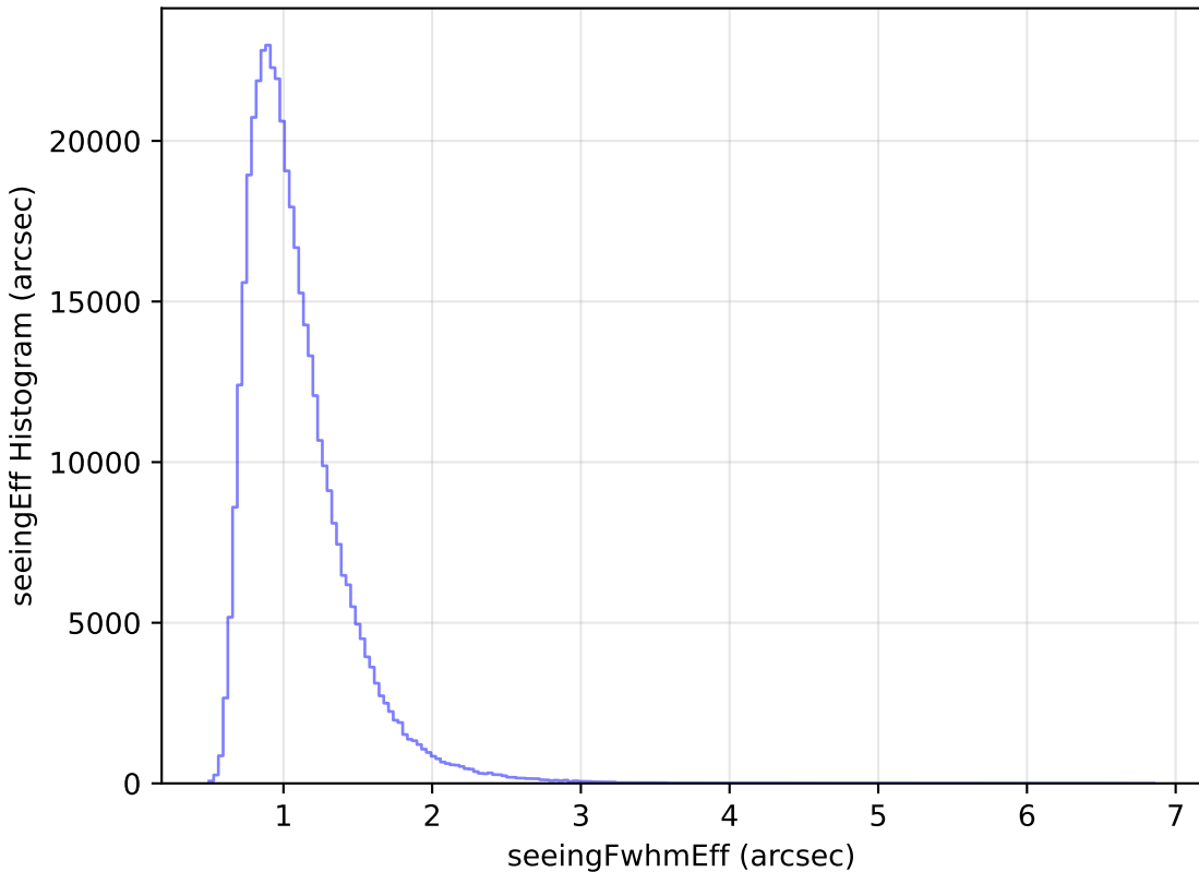
internal_u_expt27_nscale1.2v3.4_10yrs WFD z band: seeingEff Histogram
