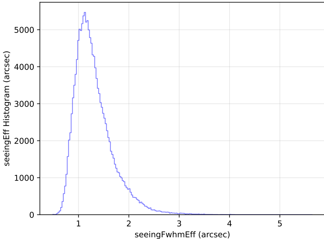
internal_u_expt27_nscale1.2v3.4_10yrs WFD u band: seeingEff Histogram
