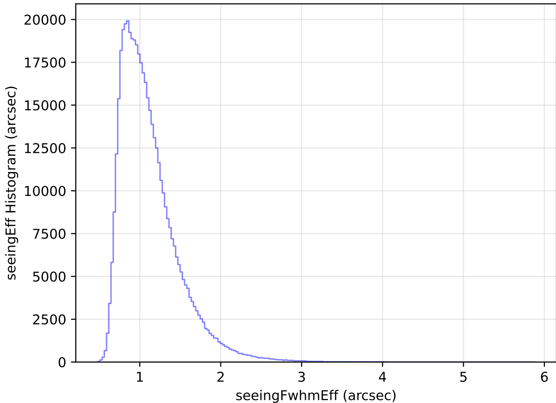
internal_u_expt27_nscale1.2v3.4_10yrs WFD r band: seeingEff Histogram
