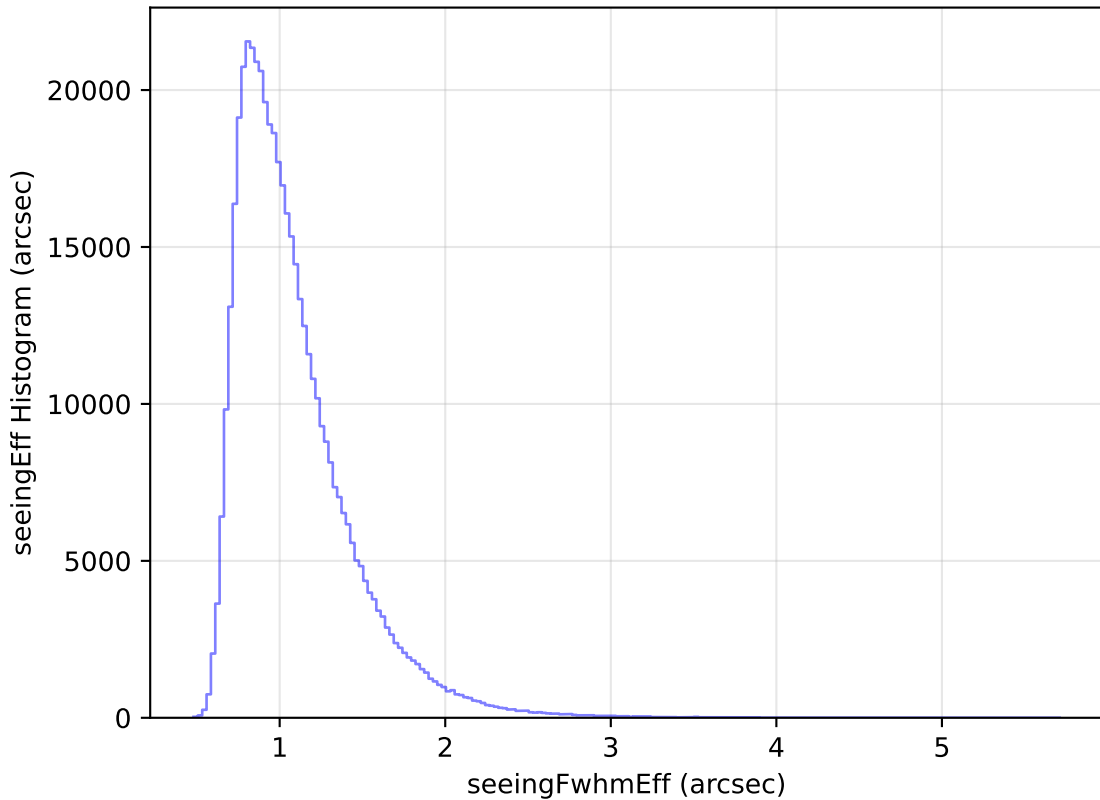
internal_u_expt27_nscale1.2v3.4_10yrs WFD i band: seeingEff Histogram
