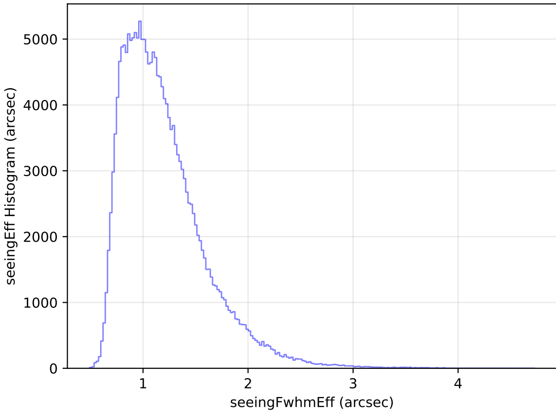
internal_u_expt27_nscale1.2v3.4_10yrs WFD g band: seeingEff Histogram
