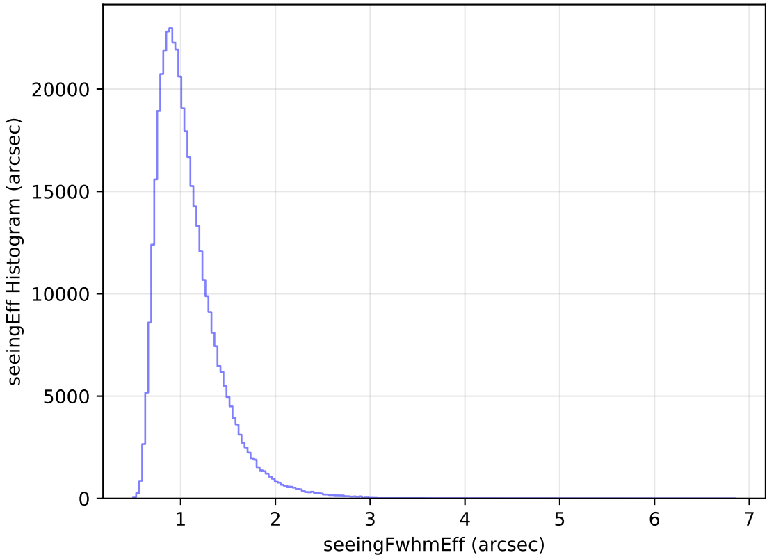
internal_u_expt27_nscale1.2v3.4_10yrs All sky z band: seeingEff Histogram
