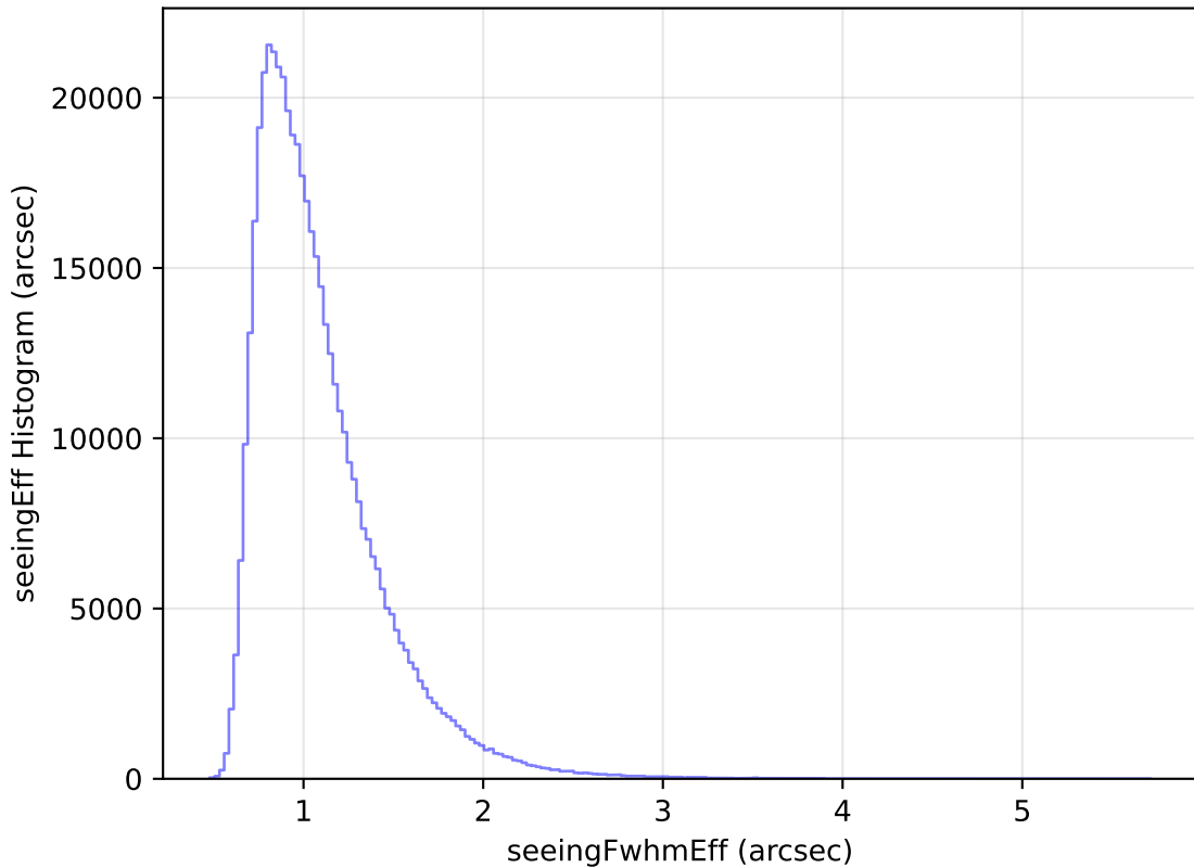
internal_u_expt27_nscale1.2v3.4_10yrs All sky i band: seeingEff Histogram
