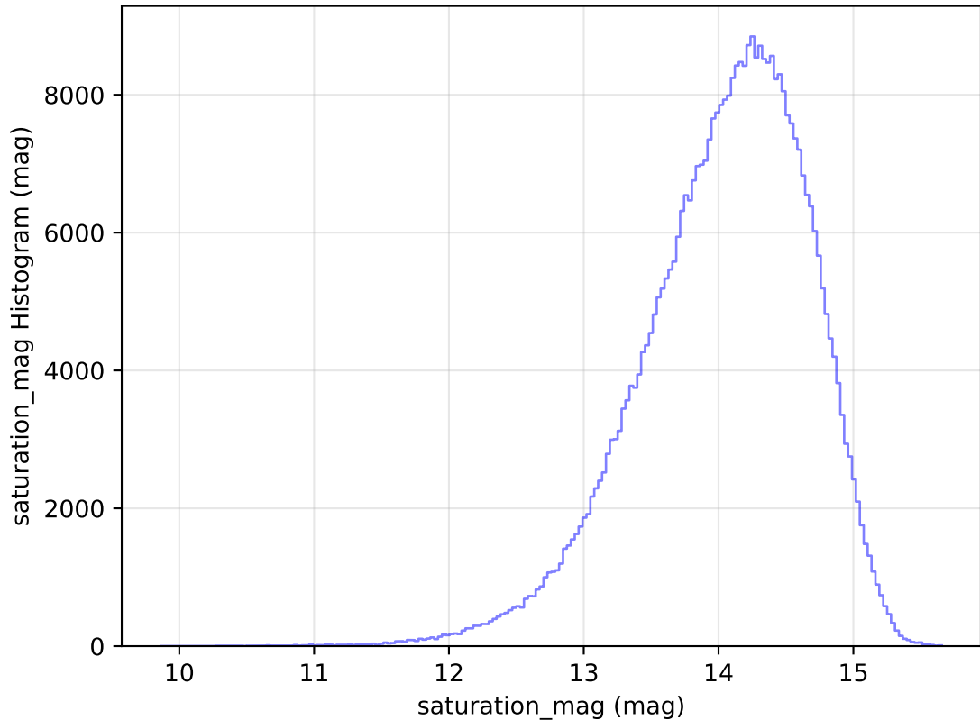
internal_u_expt27_nscale1.2v3.4_10yrs WFD z band: saturation_mag Histogram
