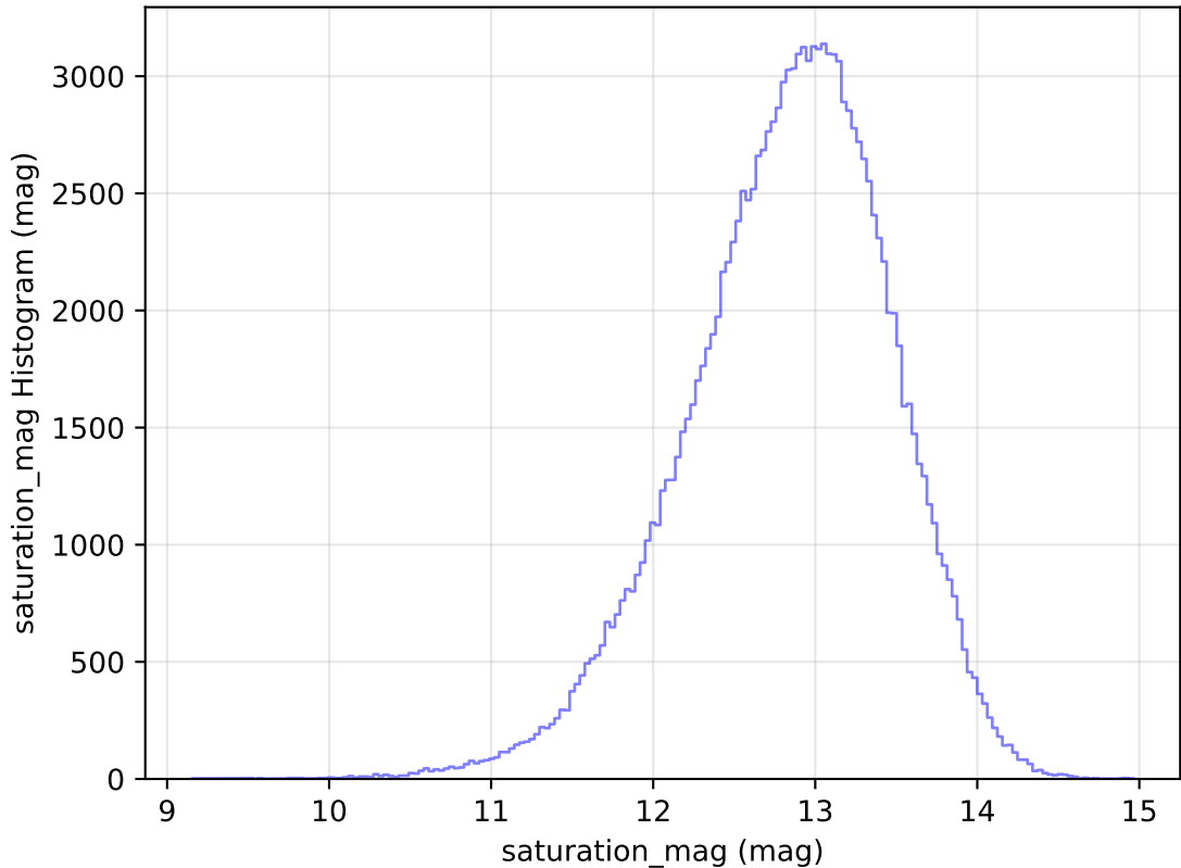
internal_u_expt27_nscale1.2v3.4_10yrs WFD u band: saturation_mag Histogram
