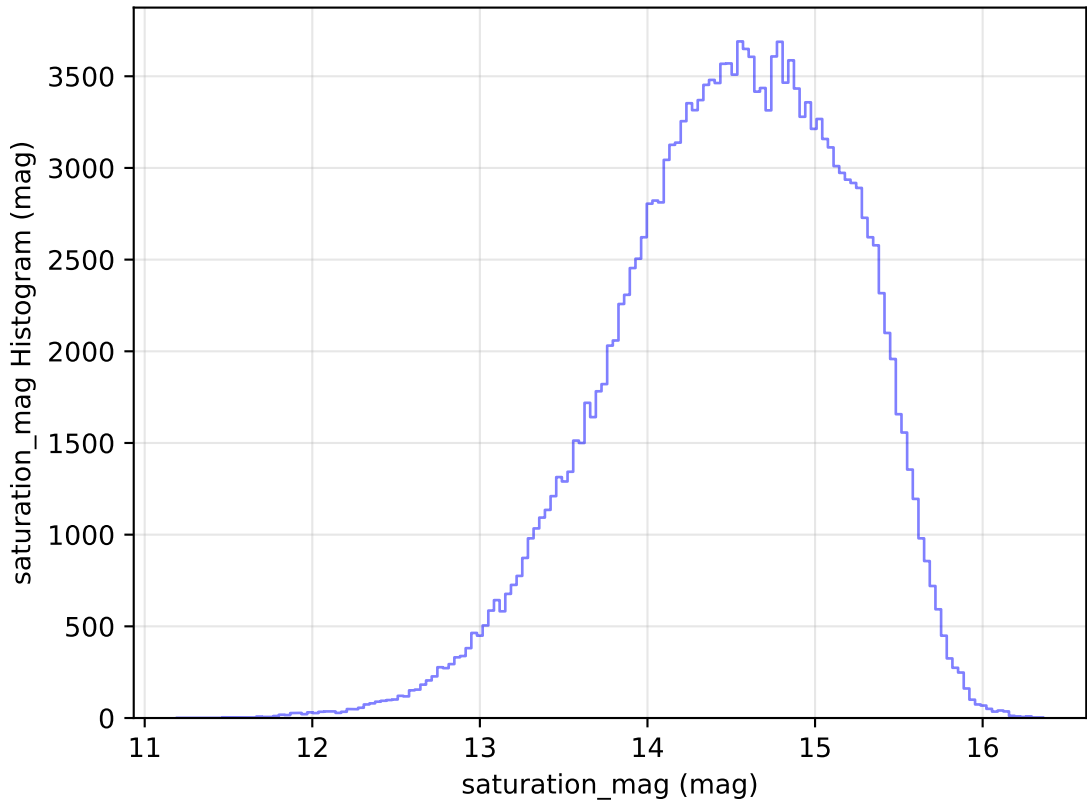
internal_u_expt27_nscale1.2v3.4_10yrs WFD g band: saturation_mag Histogram
