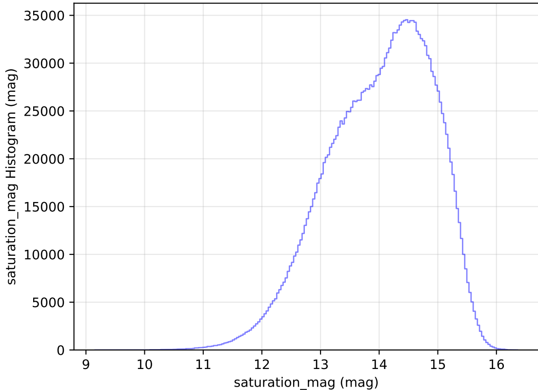
internal_u_expt27_nscale1.2v3.4_10yrs WFD all bands: saturation_mag Histogram
