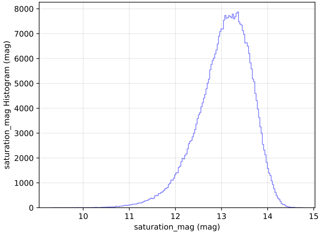
internal_u_expt27_nscale1.2v3.4_10yrs All sky y band: saturation_mag Histogram
