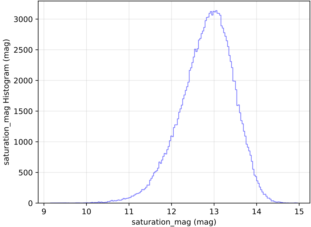
internal_u_expt27_nscale1.2v3.4_10yrs All sky u band: saturation_mag Histogram
