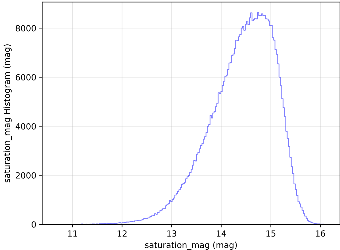
internal_u_expt27_nscale1.2v3.4_10yrs All sky i band: saturation_mag Histogram
