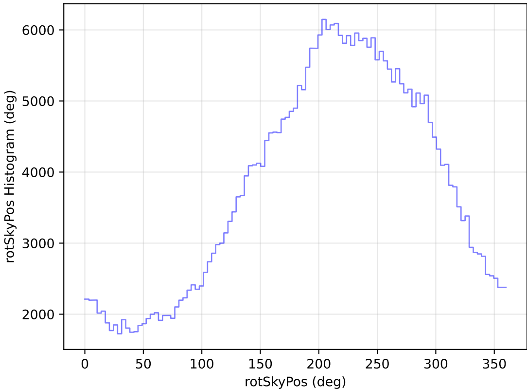
internal_u_expt27_nscale1.2v3.4_10yrs WFD y band: rotSkyPos Histogram
