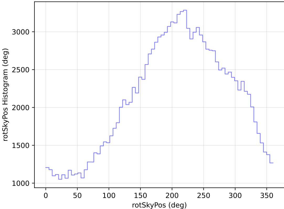
internal_u_expt27_nscale1.2v3.4_10yrs WFD u band: rotSkyPos Histogram
