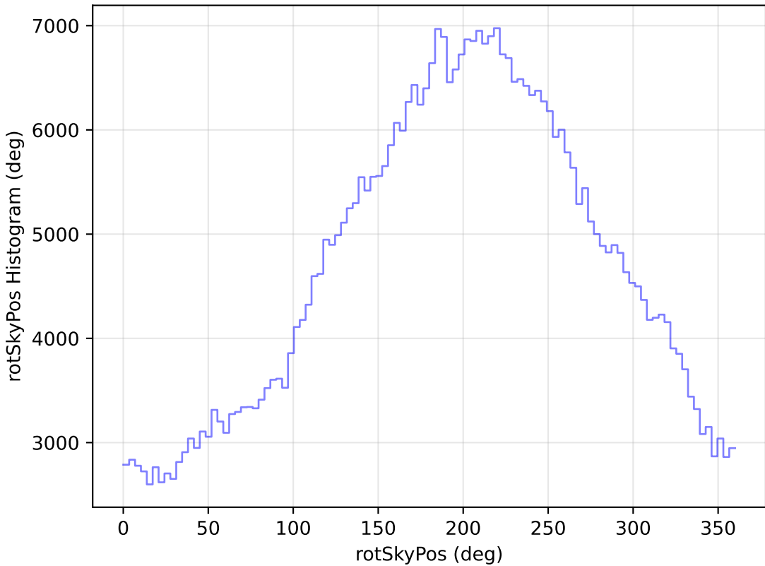
internal_u_expt27_nscale1.2v3.4_10yrs WFD r band: rotSkyPos Histogram
