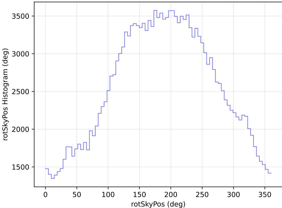
internal_u_expt27_nscale1.2v3.4_10yrs WFD g band: rotSkyPos Histogram
