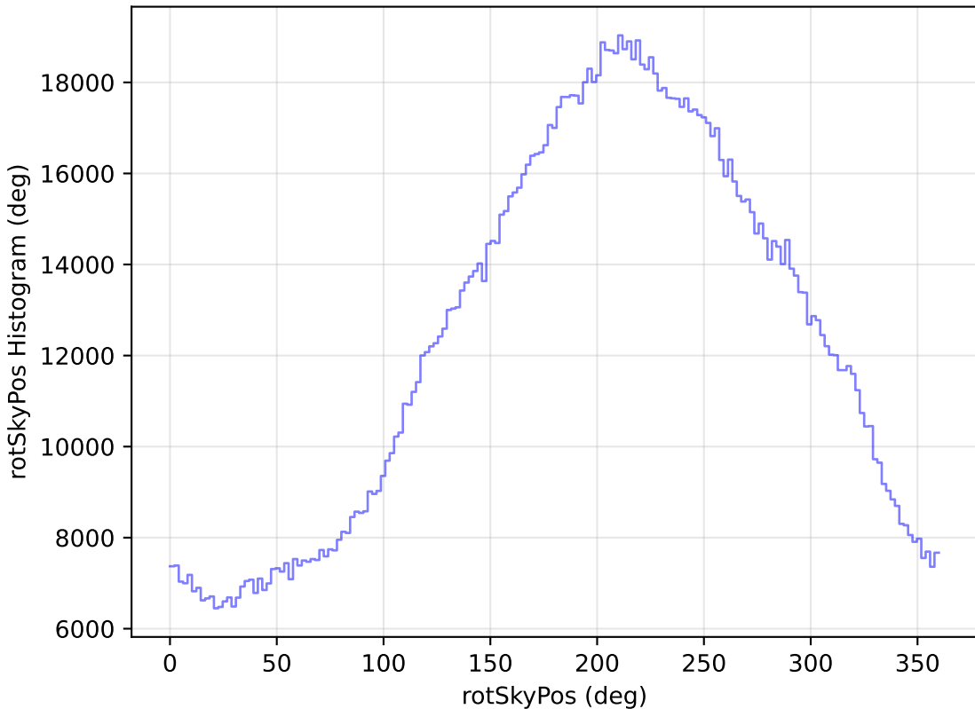
internal_u_expt27_nscale1.2v3.4_10yrs WFD all bands: rotSkyPos Histogram
