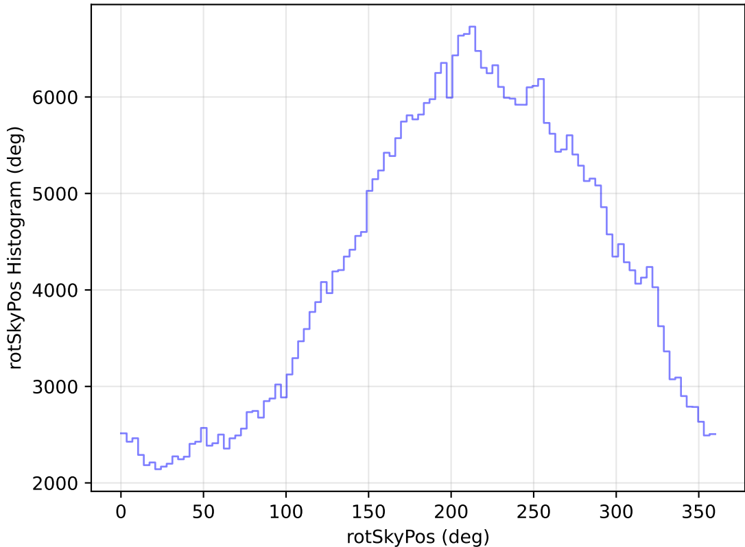
internal_u_expt27_nscale1.2v3.4_10yrs All sky z band: rotSkyPos Histogram
