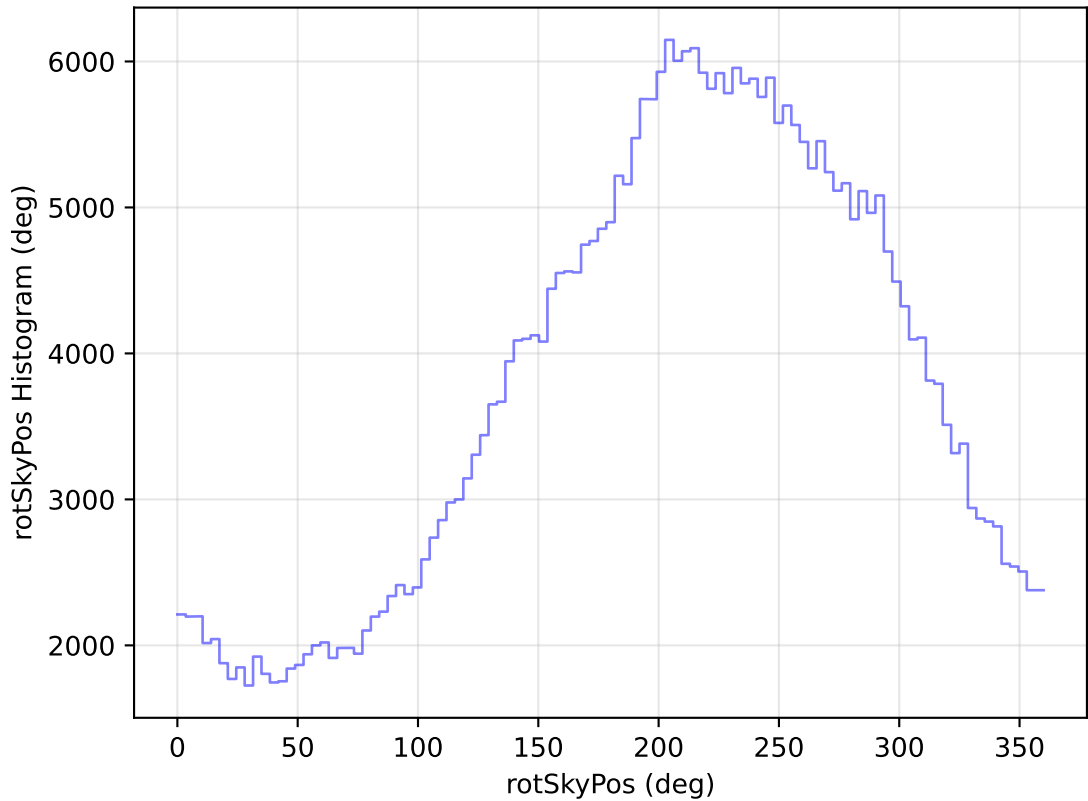
internal_u_expt27_nscale1.2v3.4_10yrs All sky y band: rotSkyPos Histogram
