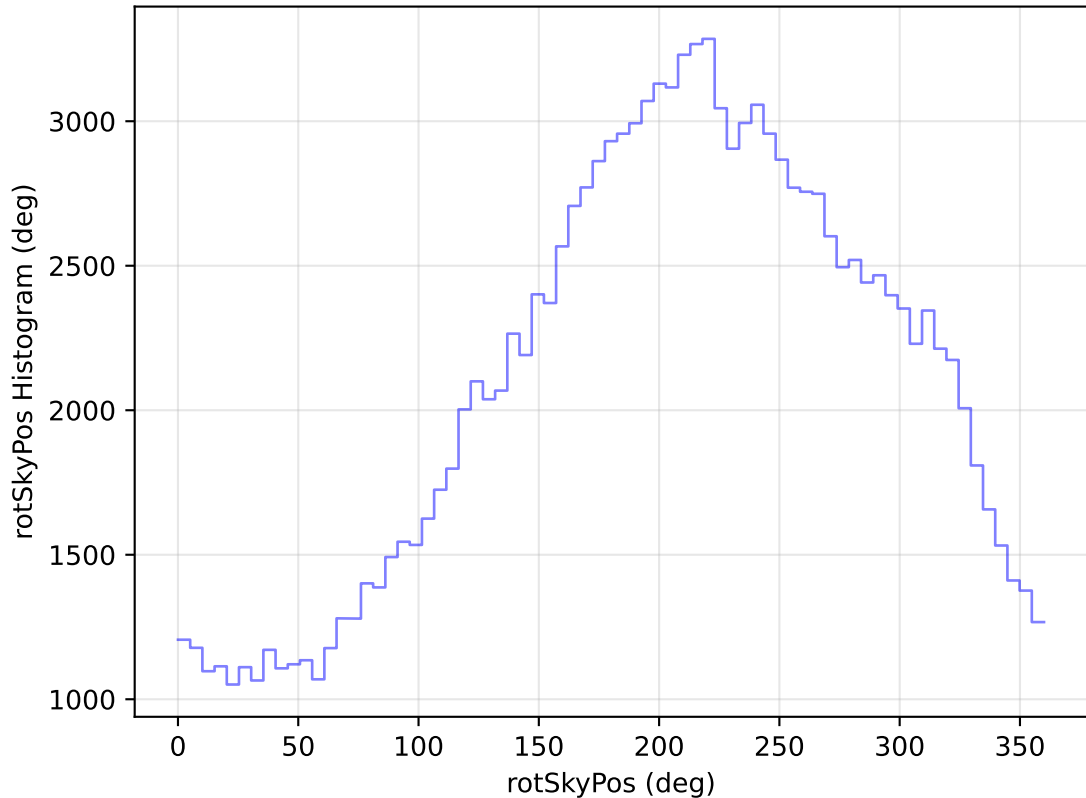
internal_u_expt27_nscale1.2v3.4_10yrs All sky u band: rotSkyPos Histogram
