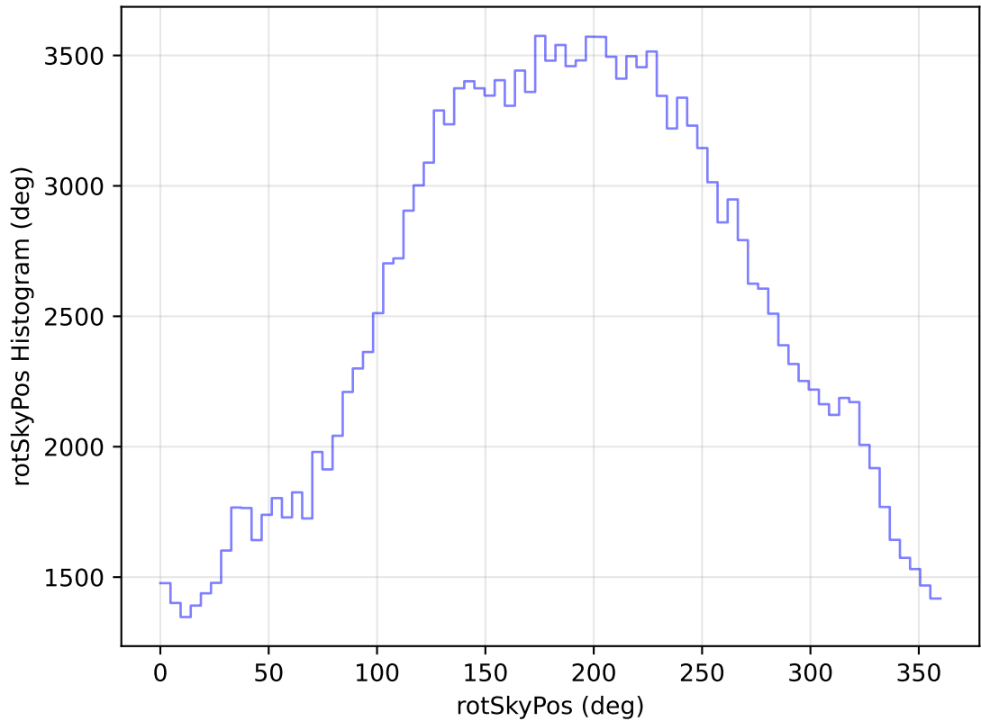
internal_u_expt27_nscale1.2v3.4_10yrs All sky g band: rotSkyPos Histogram
