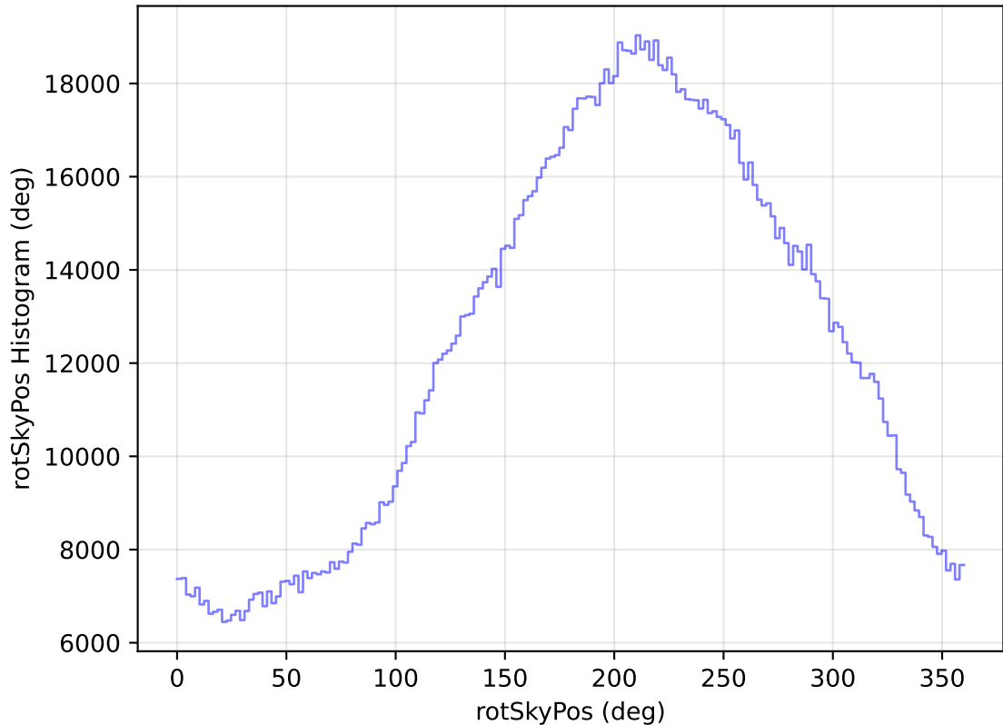
internal_u_expt27_nscale1.2v3.4_10yrs All sky all bands: rotSkyPos Histogram
