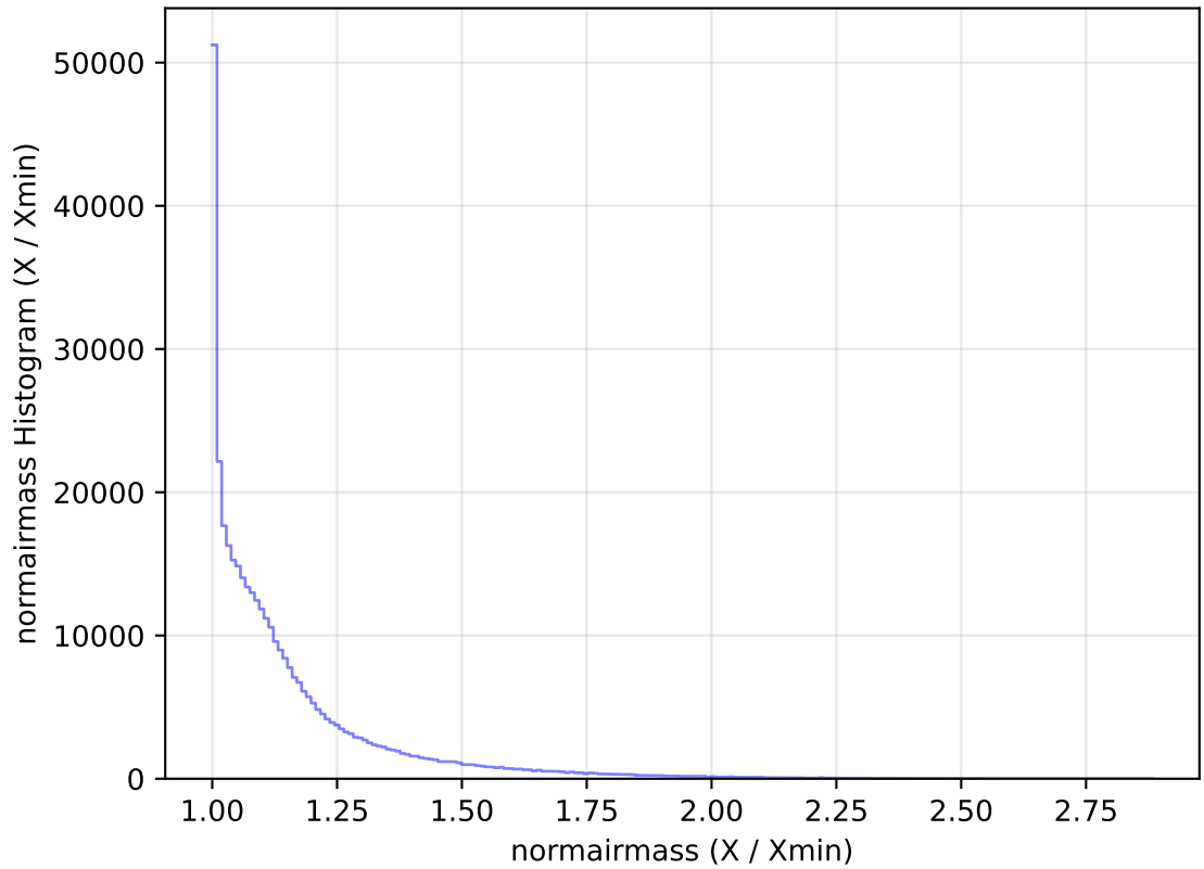
internal_u_expt27_nscale1.2v3.4_10yrs WFD y band: normairmass Histogram
