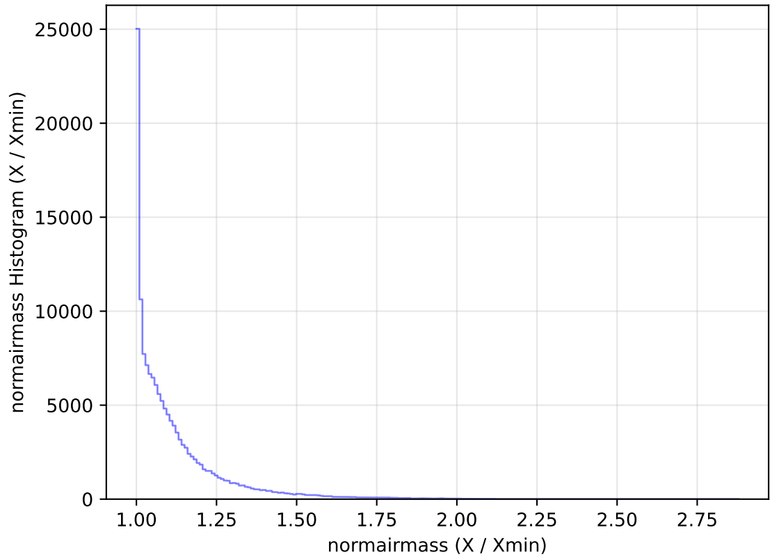
internal_u_expt27_nscale1.2v3.4_10yrs WFD u band: normairmass Histogram
