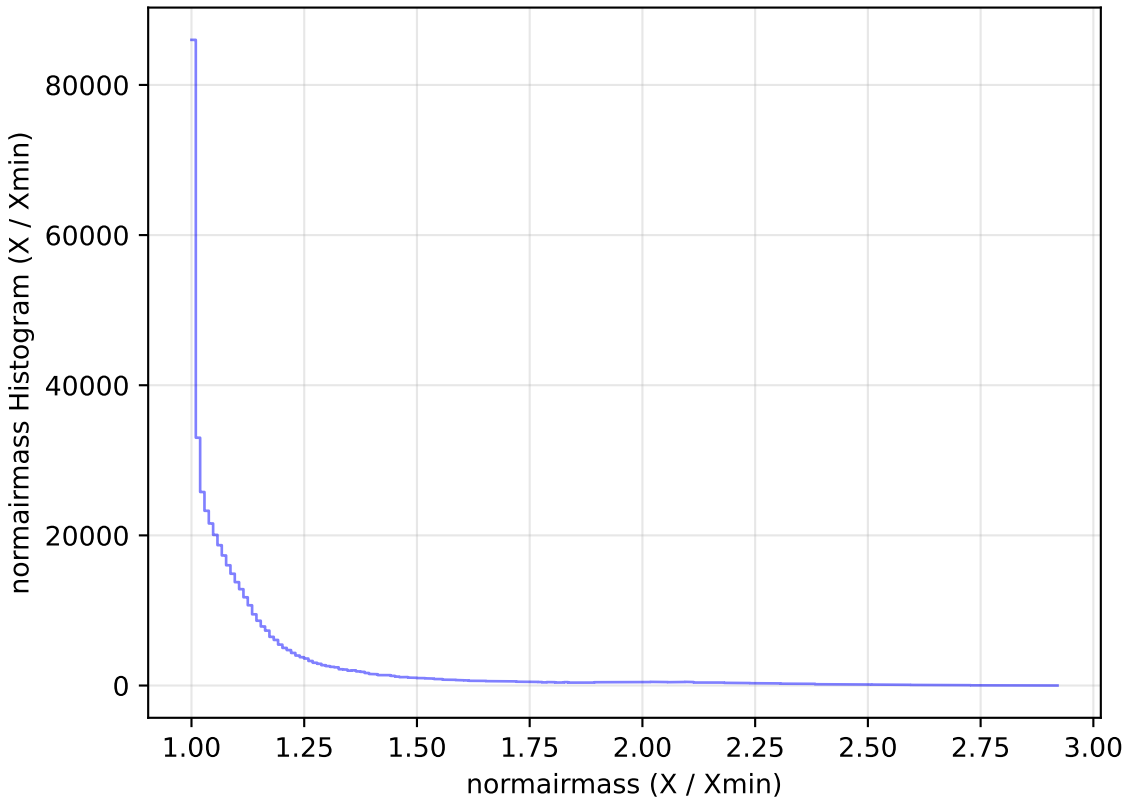
internal_u_expt27_nscale1.2v3.4_10yrs WFD i band: normairmass Histogram
