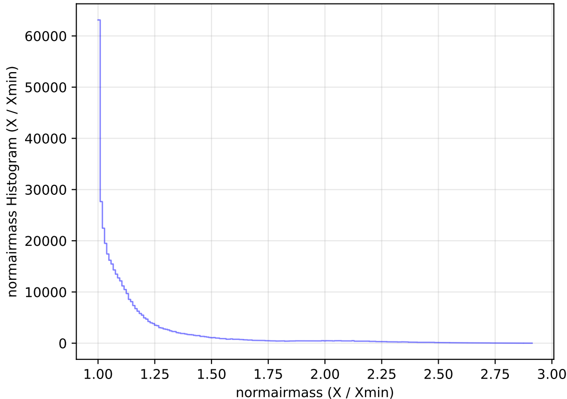
internal_u_expt27_nscale1.2v3.4_10yrs All sky z band: normairmass Histogram
