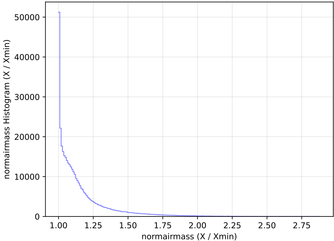
internal_u_expt27_nscale1.2v3.4_10yrs All sky y band: normairmass Histogram
