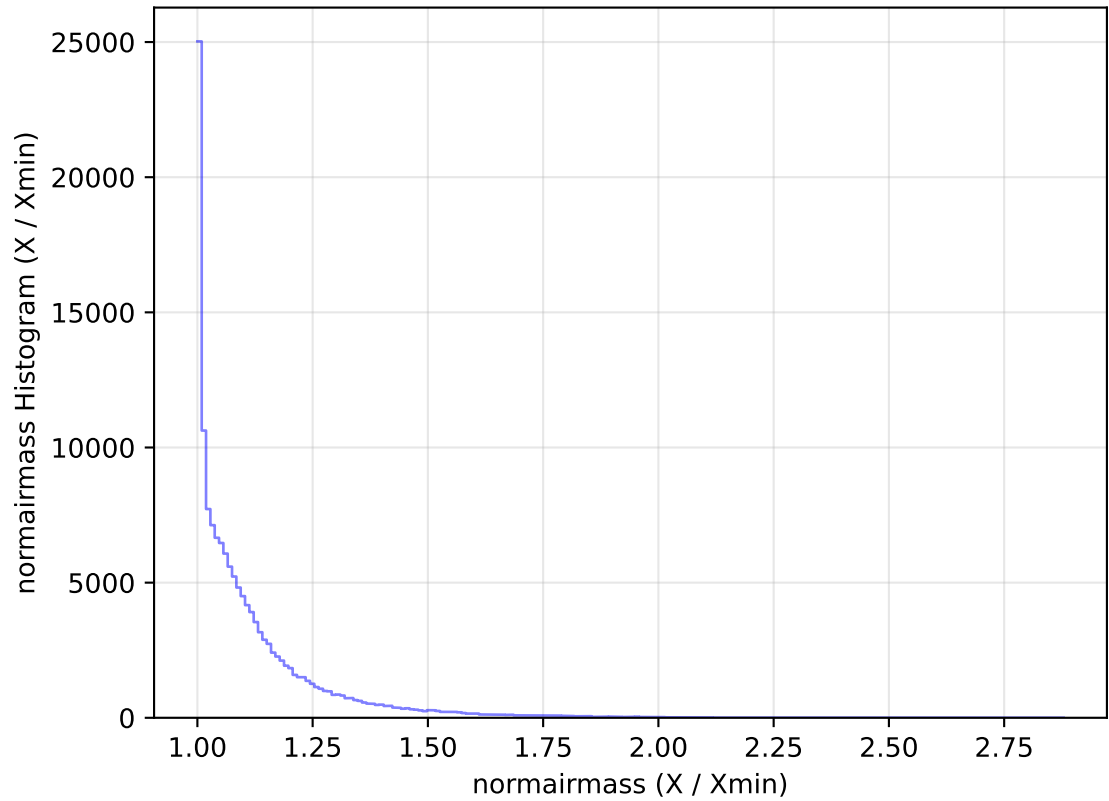
internal_u_expt27_nscale1.2v3.4_10yrs All sky u band: normairmass Histogram
