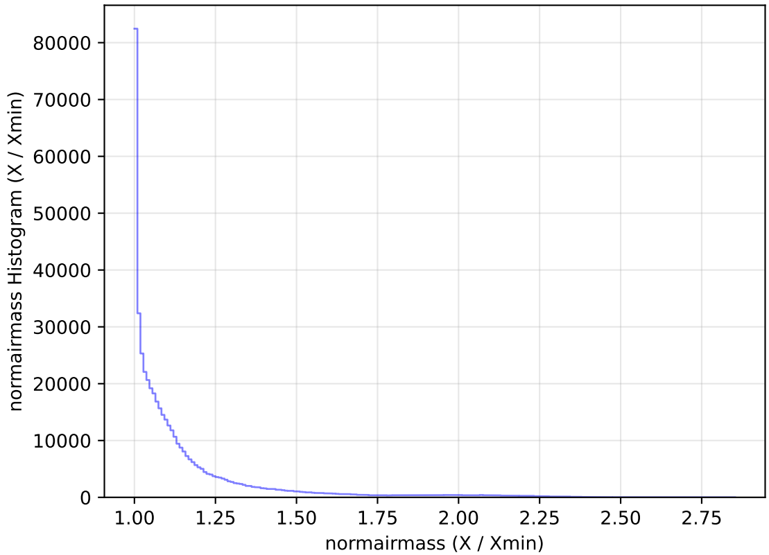
internal_u_expt27_nscale1.2v3.4_10yrs All sky r band: normairmass Histogram
