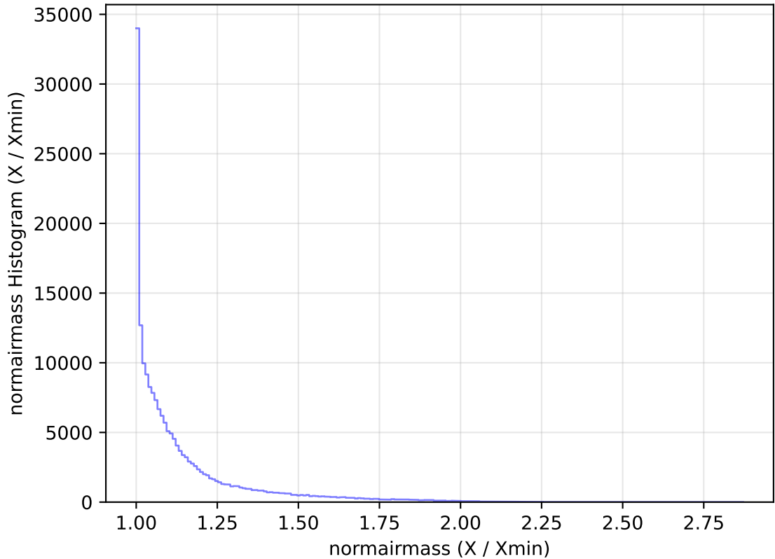
internal_u_expt27_nscale1.2v3.4_10yrs All sky g band: normairmass Histogram
