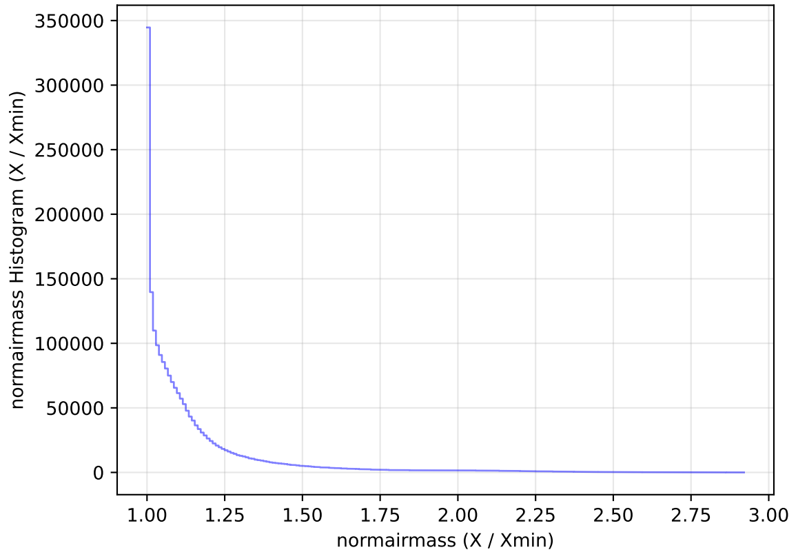
internal_u_expt27_nscale1.2v3.4_10yrs All sky all bands: normairmass Histogram
