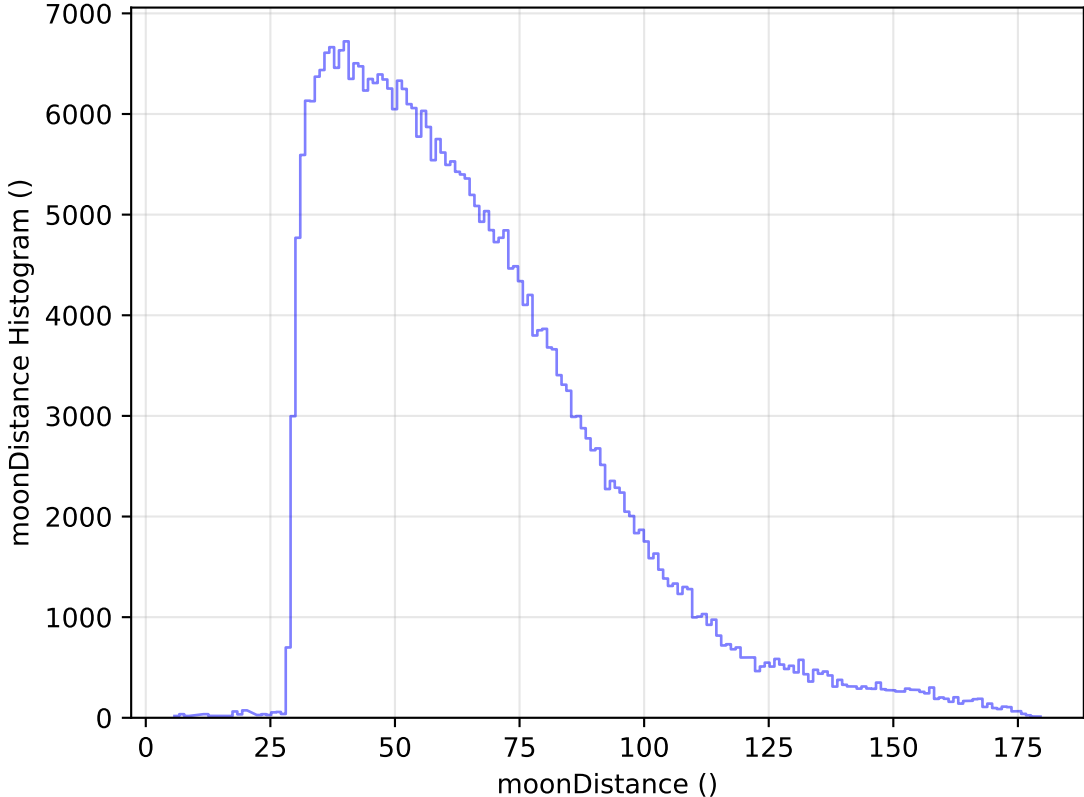
internal_u_expt27_nscale1.2v3.4_10yrs WFD y band: moonDistance Histogram
