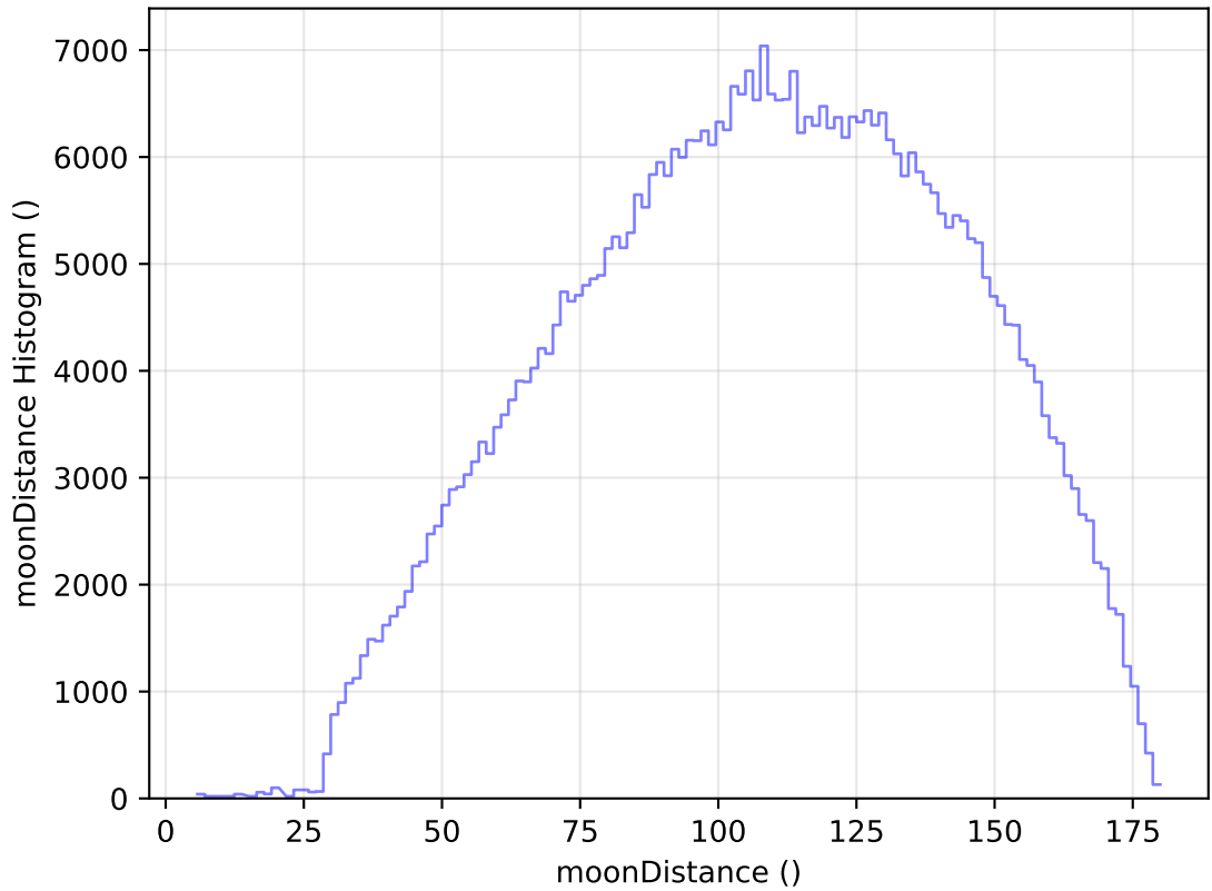
internal_u_expt27_nscale1.2v3.4_10yrs WFD r band: moonDistance Histogram
