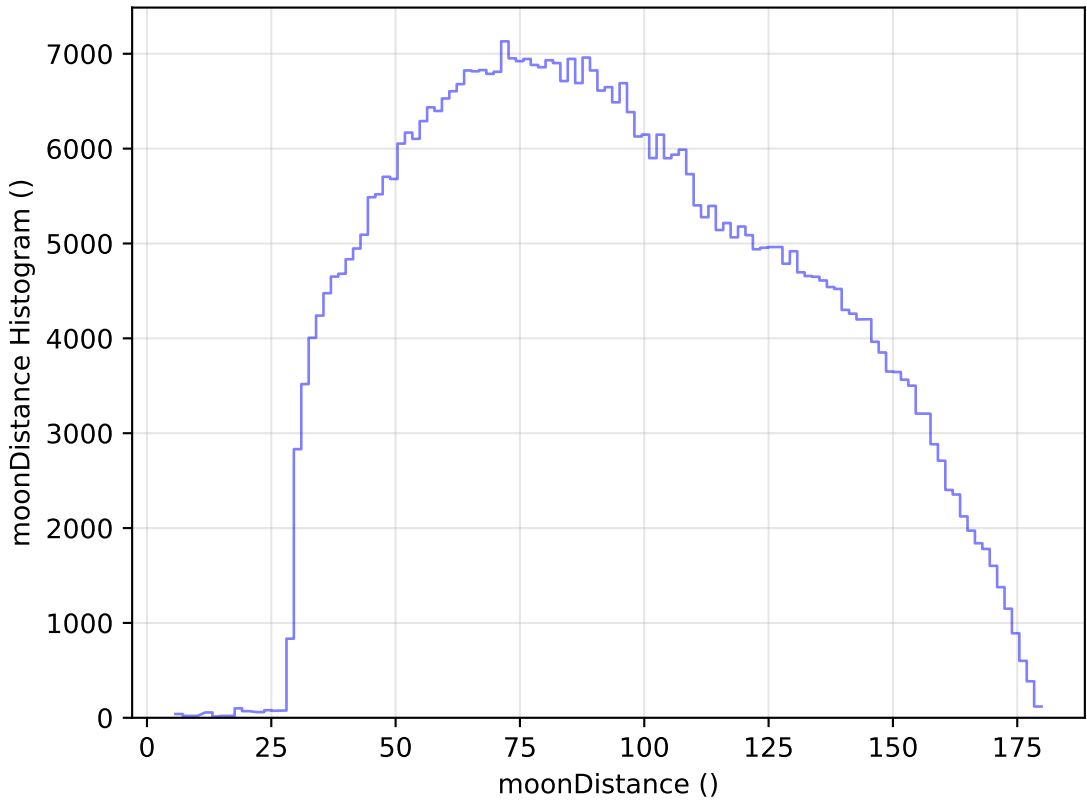
internal_u_expt27_nscale1.2v3.4_10yrs WFD i band: moonDistance Histogram
