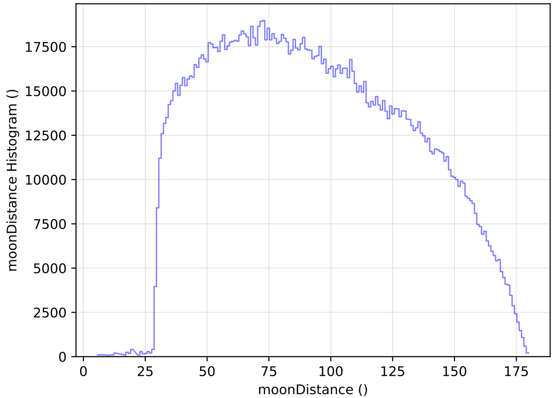
internal_u_expt27_nscale1.2v3.4_10yrs WFD all bands: moonDistance Histogram
