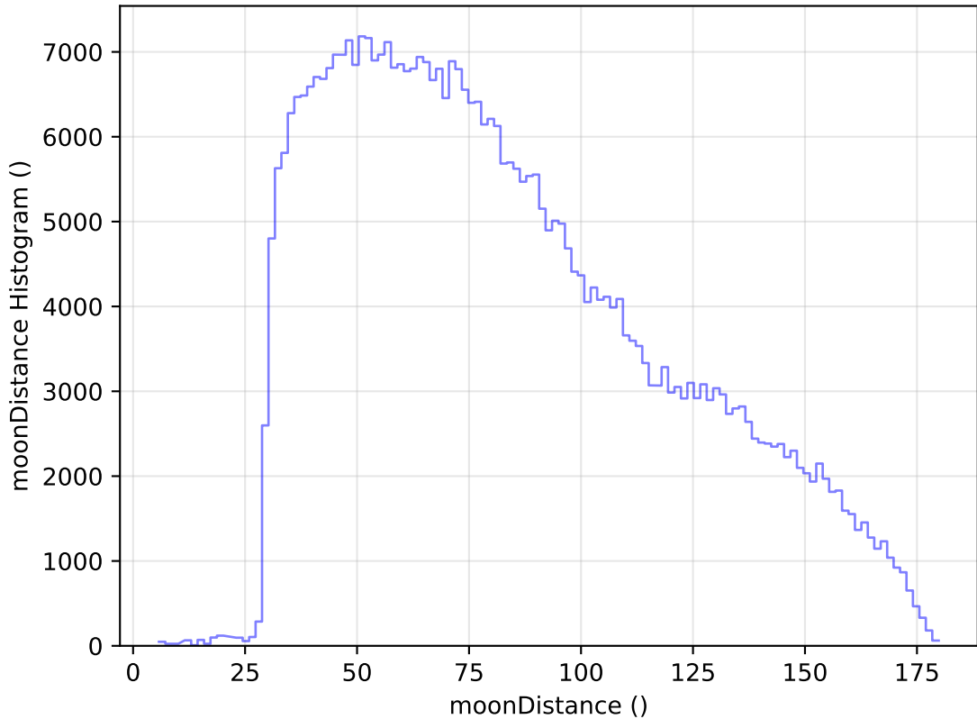
internal_u_expt27_nscale1.2v3.4_10yrs All sky z band: moonDistance Histogram
