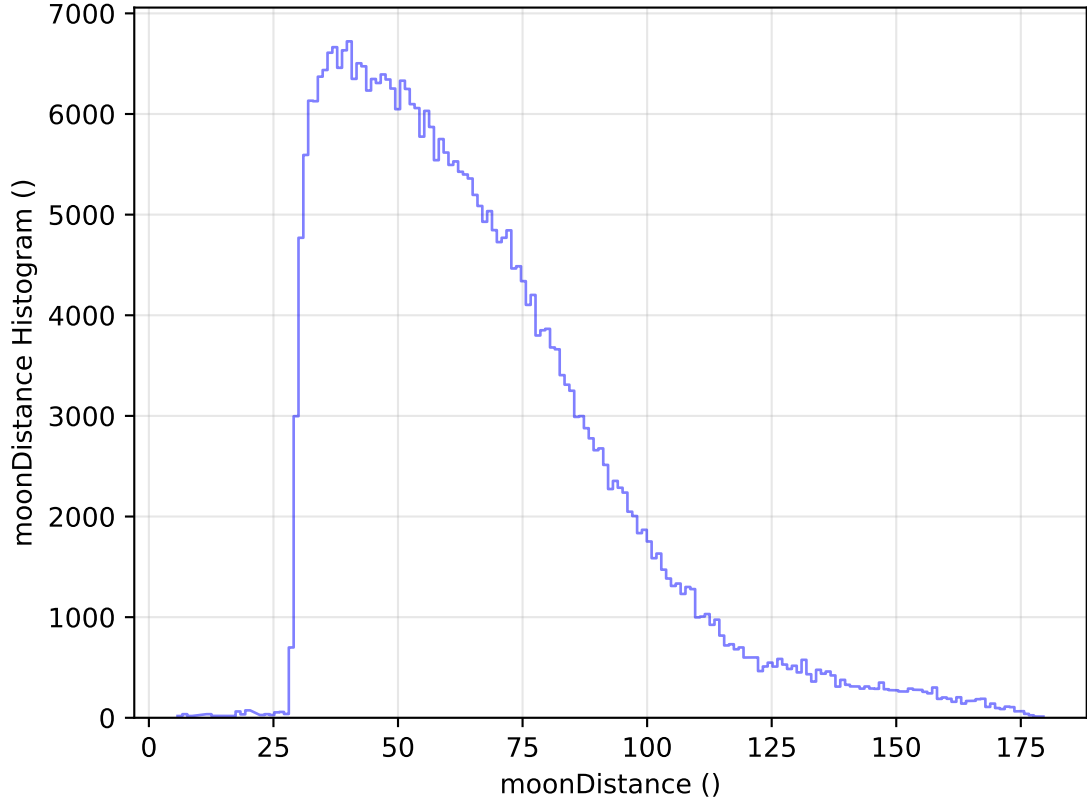
internal_u_expt27_nscale1.2v3.4_10yrs All sky y band: moonDistance Histogram
