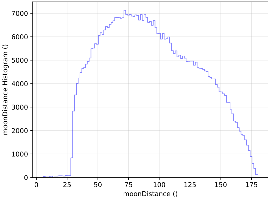
internal_u_expt27_nscale1.2v3.4_10yrs All sky i band: moonDistance Histogram
