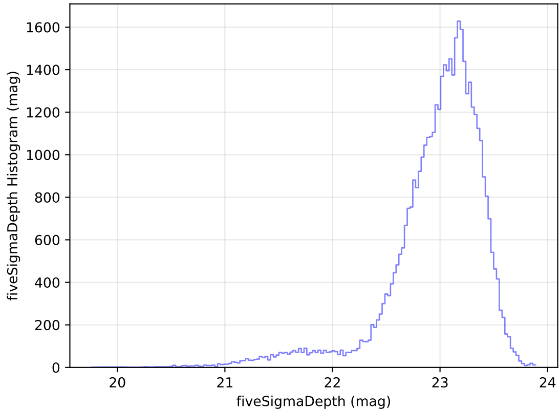
internal_u_expt27_nscale1.2v3.4_10yrs Yr 1 z band: fiveSigmaDepth Histogram
