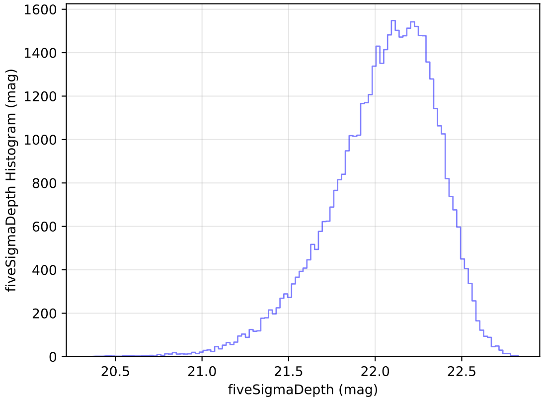
internal_u_expt27_nscale1.2v3.4_10yrs Yr 1 y band: fiveSigmaDepth Histogram
