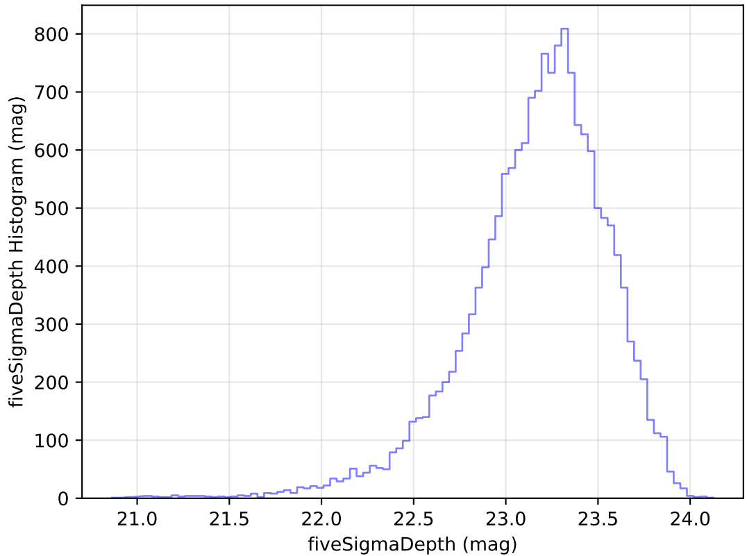
internal_u_expt27_nscale1.2v3.4_10yrs Yr 1 u band: fiveSigmaDepth Histogram
